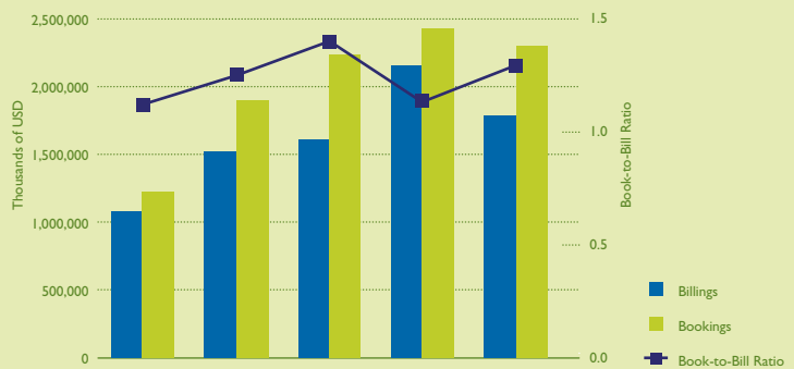
WORLDWIDE PV MANUFACTURING EQUIPMENT BOOKINGS, BILLINGS, AND BOOK-TO-BILL RATIO
